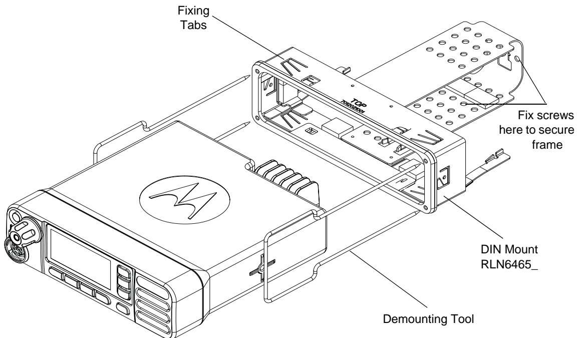
Figure 2-9 Dashboard Mounting for MOTOTRBO XPR 4000 Series
