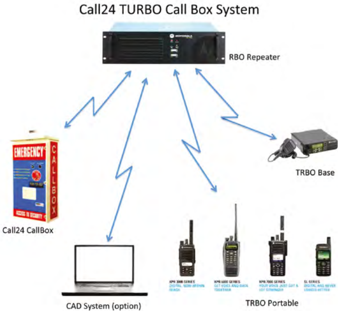
CALL24 Wireless TRBO Call Box
